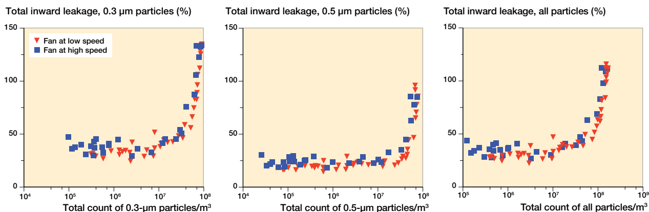
Figure 4. Scatterplots of percentage total inward leakage versus total count of 0.3 μm, 0.5 μm, and all particle sizes per m 3 .
